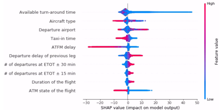
Figure 1. Top 10 most important features
