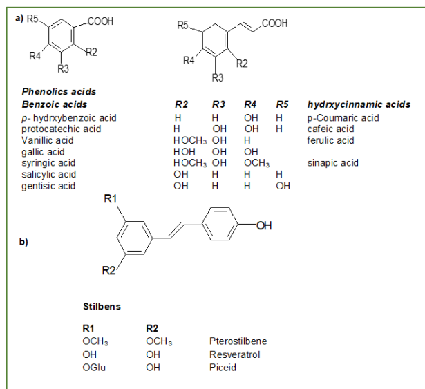
Figure 4: (a) Structure of grape phenolic acids and (b) Chemical structures of some grape stilbene [23, 24]
