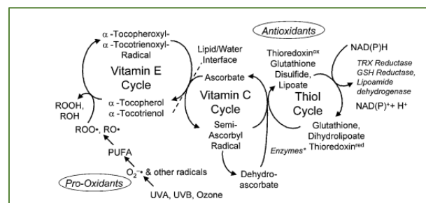
Figure 2: Tocopherols regeneration via the ascorbic acid action [17]
